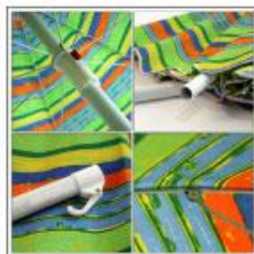
HT-BE011 Size:115*8K Fabric:TNT Ribs:3.2mm white steel ribs Pole:dia 32/32mm, 125/95cm length white steel pole Tilt: plastic button tilt
